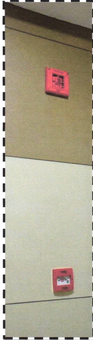
CHAVARA BLOCK- MANUAL OPERATED FIRE ALARM SYSTEM
