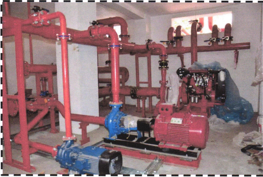
FIRE PUMP SYSTEM – CHAVARA BLOCK
