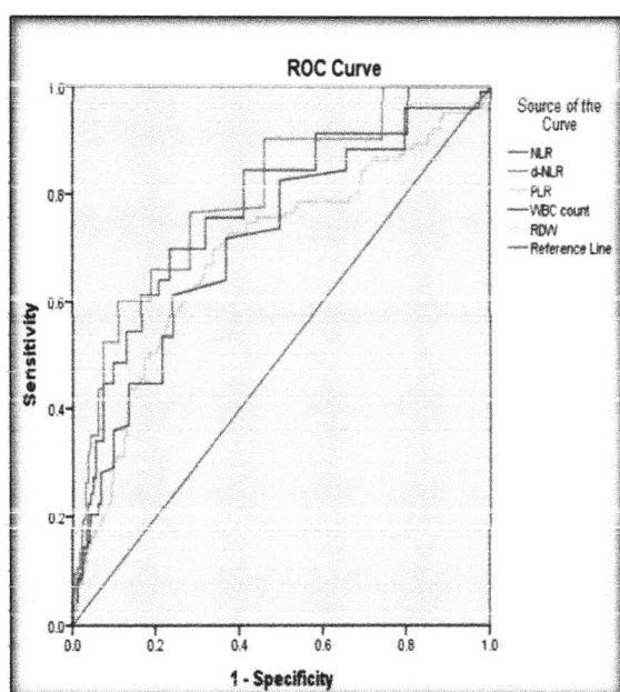
Figure 3: ROC Curve
