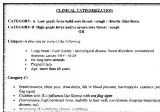
Figure 1: Clinical Categorization
